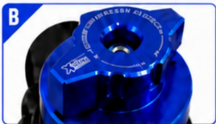
COMPRESSION DAMPING ADJUSTMENT
